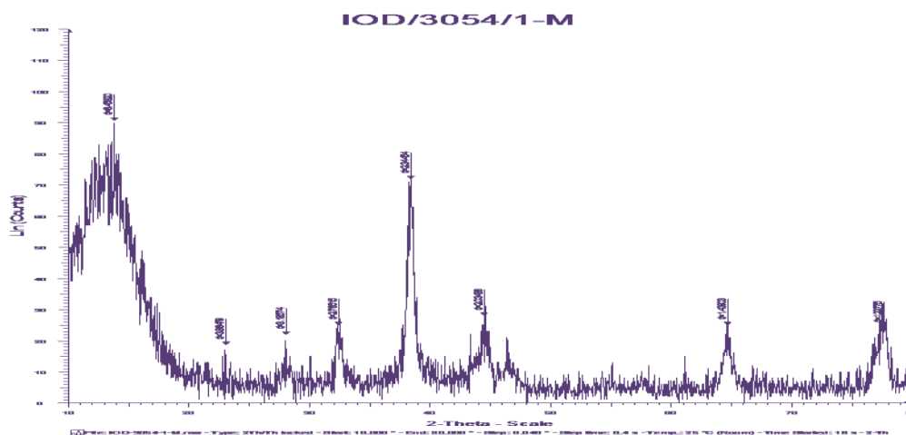
Figure 3. XRD patterns of synthesized silver nanoparticles using aqueous extract of broiler chicken faecal excreta.
