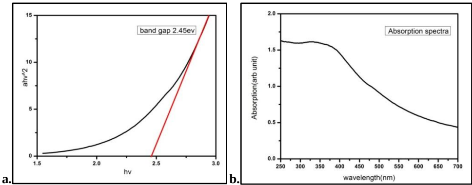
Figure 7 (a, b). Shows the UV–visible spectrum of Fe 3 O 4 nanoparticles showing an absorption band in the region of 307-345 nm.
