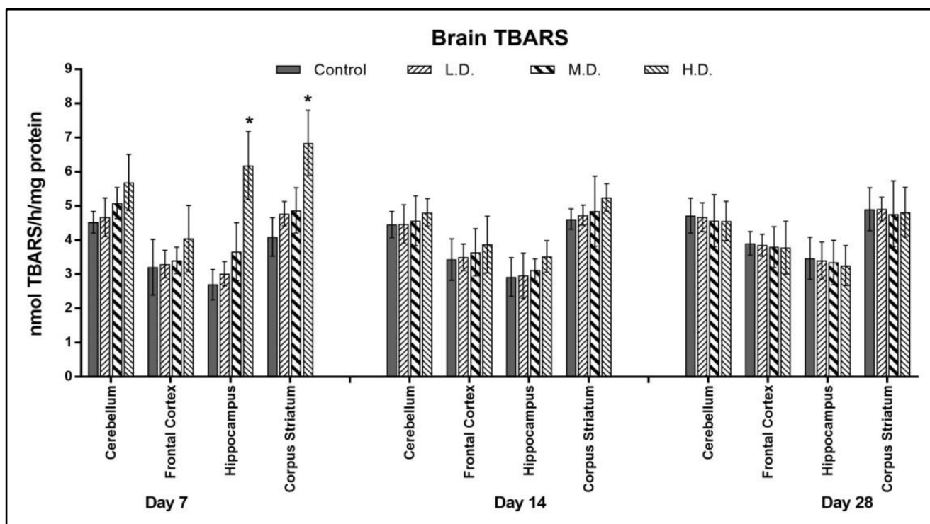
Figure 10: TBARS levels in Cerebellum, Frontal Cortex, Hippocampus and Corpus Striatum of rats following administration of IONP. Each group contained 6 animals and values represented as mean \pm SEM. Data analyzed by one way ANOVA followed by dunnet's multiple comparison test. Abbreviations and concentration used TBARS, Thiobarbituric Acid Reactive Substances as nmol/h/mg protein. * P \leq 0.05 indicates statistical difference from Control group.
