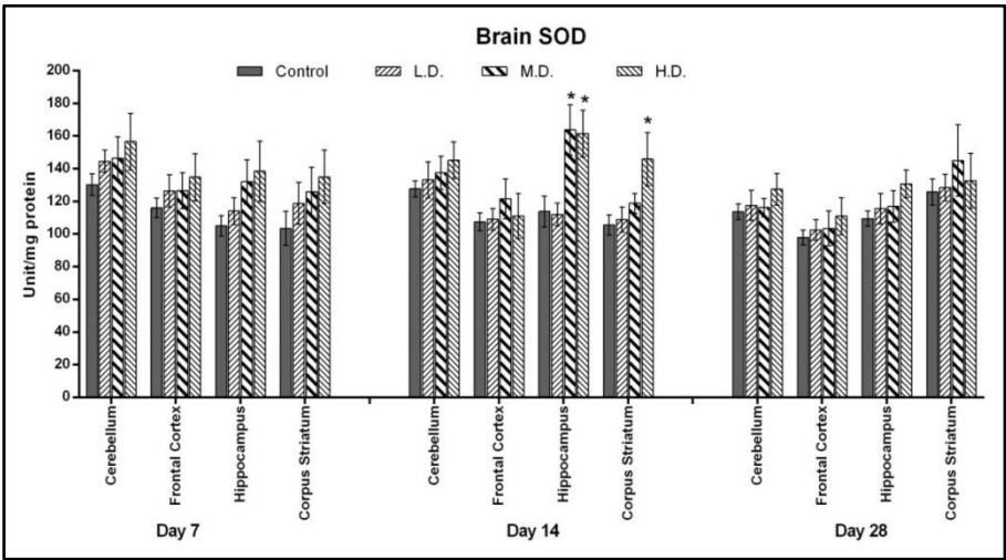
Figure 8: SOD activity in Cerebellum, Frontal Cortex, Hippocampus and Corpus Striatum of rats following administration of IONP. Each group contained 6 animals and values represented as mean ± SEM. Data analyzed by one way ANNOVA followed by dunnet’s multiple comparison test. Abbreviations and unit used: SOD, Superoxide Dismutase; 1 Unit is equals to the amount of enzyme inhibiting the rate of autoxidation of pyrogallol by 50%. *P≤0.05 indicates statistical difference from Control group.
