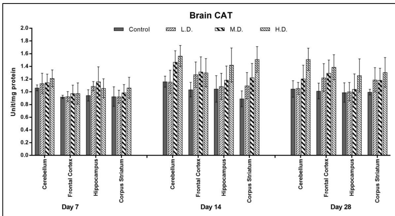
Figure 9: CAT activity in Cerebellum, Frontal Cortex, Hippocampus and Corpus Striatum of rats following administration of IONP. Each group contained 6 animals and values represented as mean \pm SEM. Data analyzed by one-way ANOVA followed by Dunnet's multiple comparison test. Abbreviations and Unit used: CAT: Catalase; 1 Unit is equals to 1 millimol H_2O_2 decomposed per minute per milligram protein.
