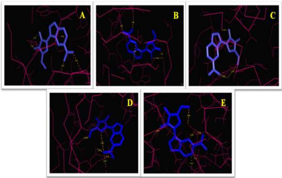
Figure 3. Visualization of docked complex with PyMol tool 2-Carbamyl-9-[Beta.-D-Ribofuranosyl.] Hypoxanthine docked with A – Caspase-3 B - Caspase-9 C - β-Actin D - p53 E - Bcl-2.
