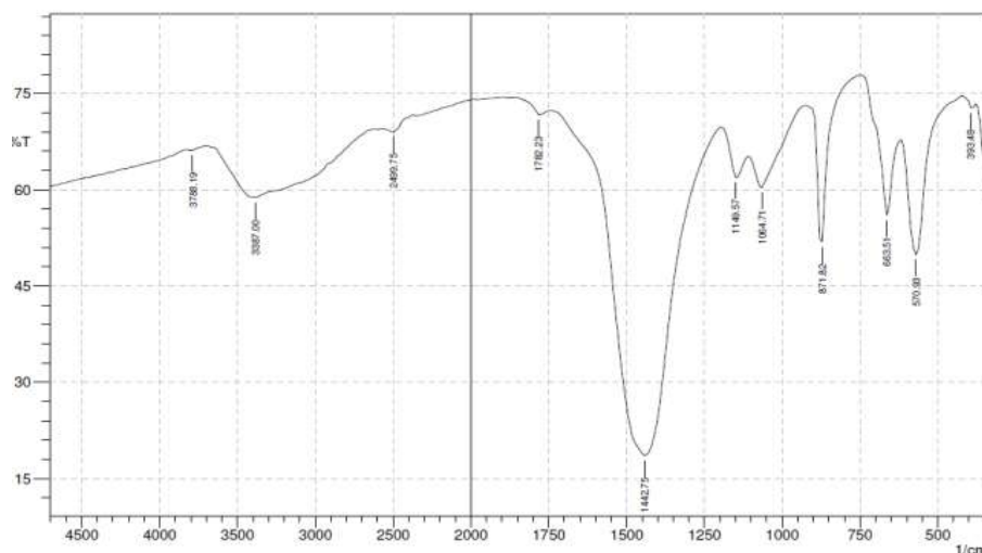
Figure 2. IR spectrum of \text{Co}_3\text{O}_4 nanoparticles.
