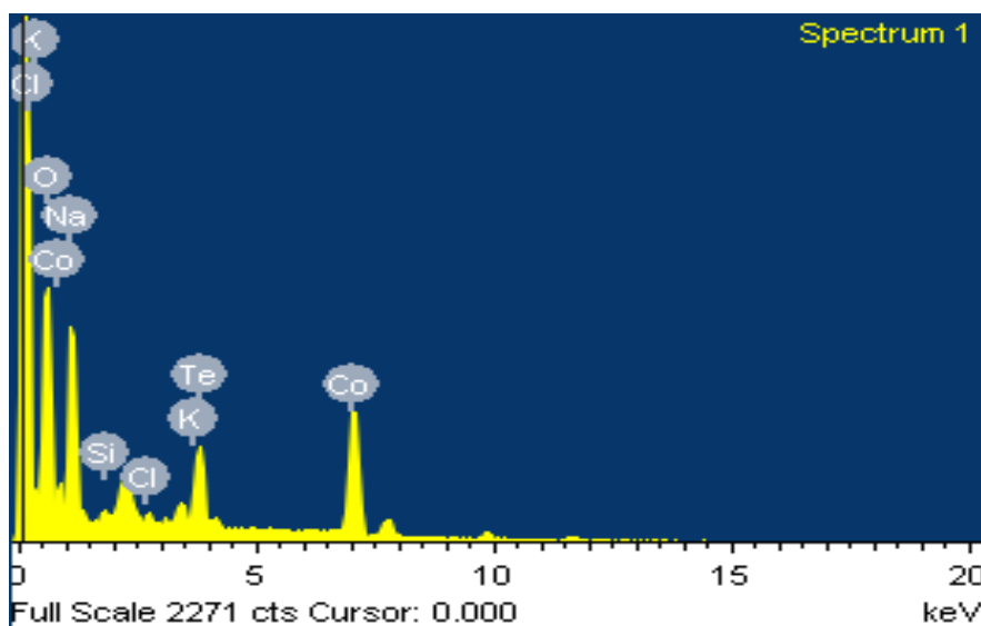
Figure 5. EDX of spectra of \text{Co}_3\text{O}_4 .
