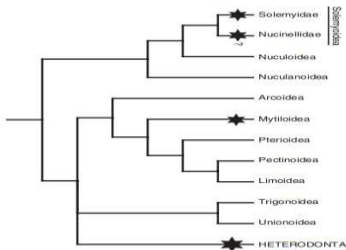
Figure 1. Phylogenetic tree of bivalve superfamilies and Heterodonta families. With star chemosymbionts and with triangle cellulolytic symbionts.
