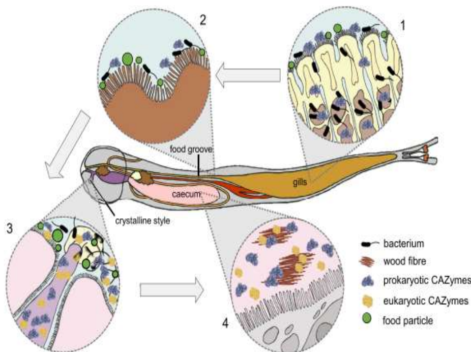
Figure 2. Digestive system of shipworms and its microbial symbiosis pathway.
