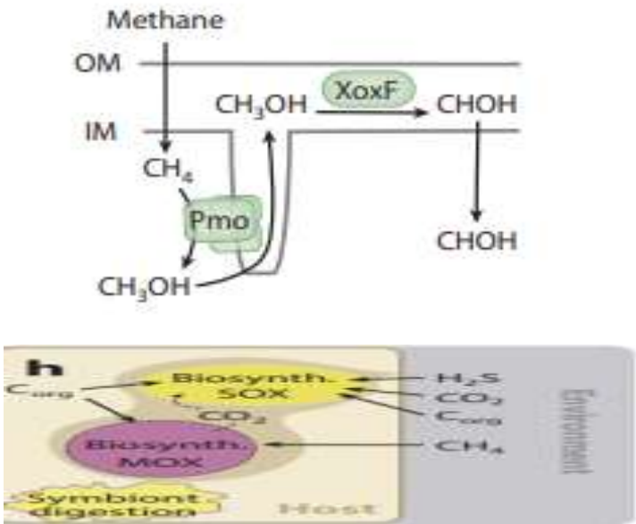
Figure 5. The metabolisms of methane oxidation (particulate methane monooxygenase a subunit).
