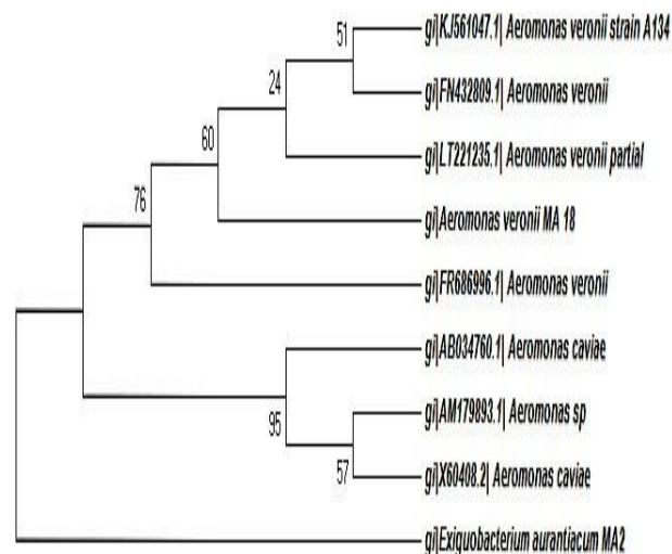
Figure 4. Phylogenetic Tree of isolated bacteria MA18.
