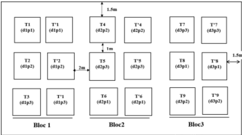
Figure 3. Experimental device
