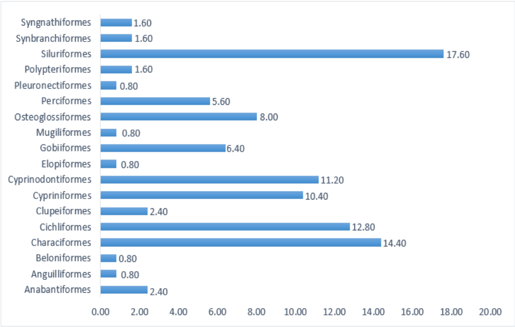
Figure 3. Numerical percentages of orders by number of species in streams
