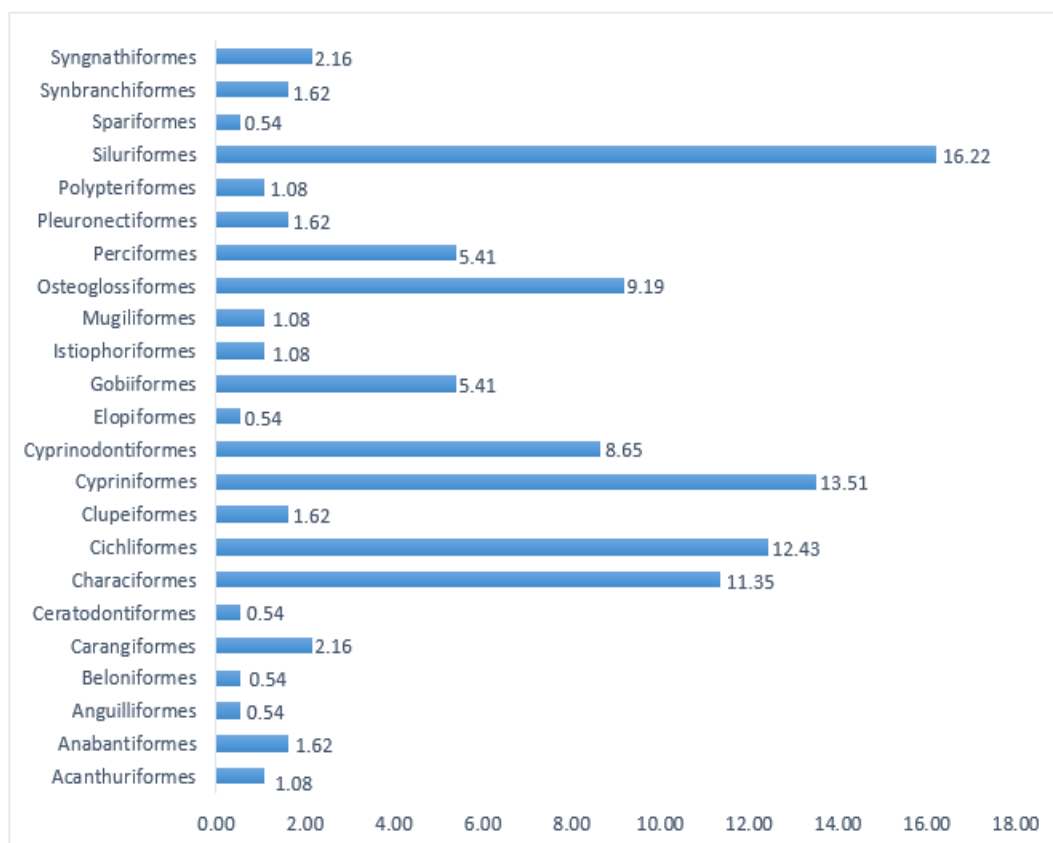
Figure 1. Numerical percentages of orders by number of species.
