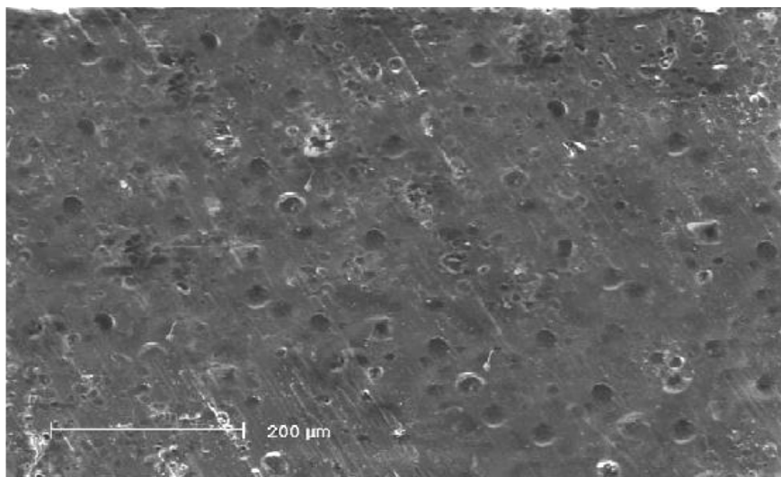
Figure 3. Scanning electron microscope (SEM) picture of EOP showing orifice size which was mechanically drilled.
