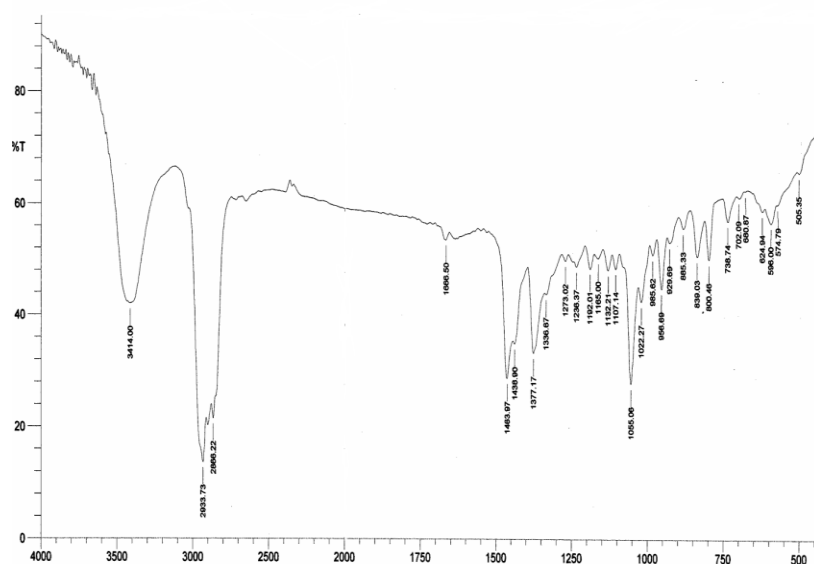
Figure 6. FTIR Spectra of Drug And Peg-400
