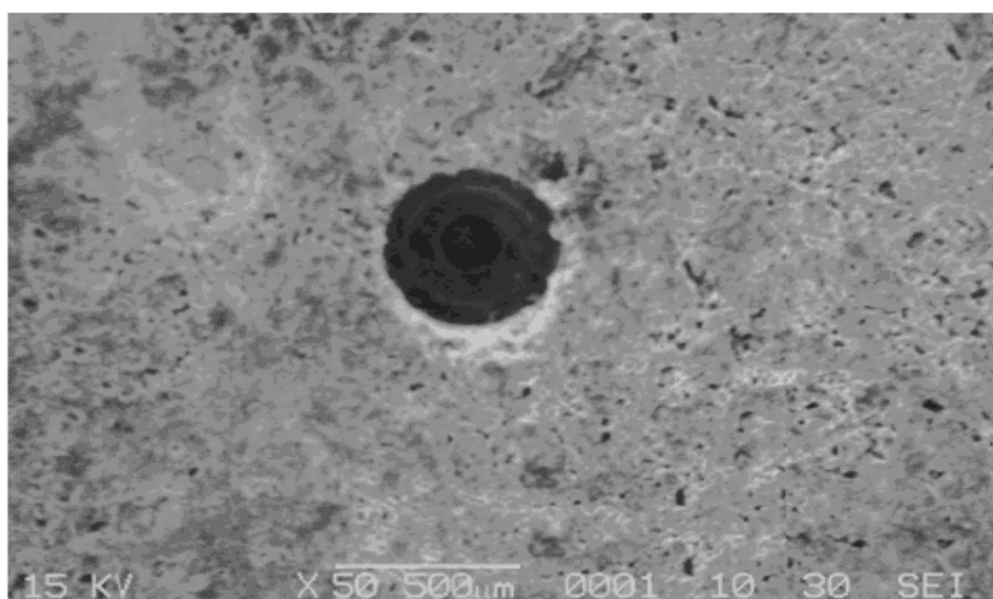
Figure 2. Scanning electron microscope (SEM) picture of EOP showing orifice size, which was mechanically drilled.
