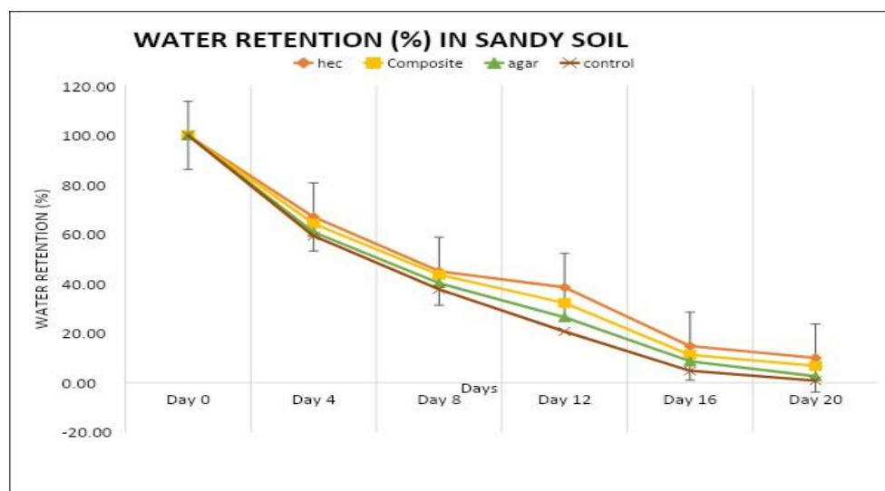
Figure 3. Water retention capacity (%) of pure sandy soil (Control) and soil containing the hydrogels Agar, Composite and HEC.
