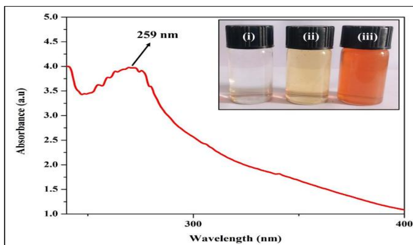
Figure: 3. UV- Visible spectrum and Chromatic variation of SeNPs after adding extract with 40 mM of sodium selenite solution (i)Sodium selenite, (ii) Extract, and (iii) SeNPs.
