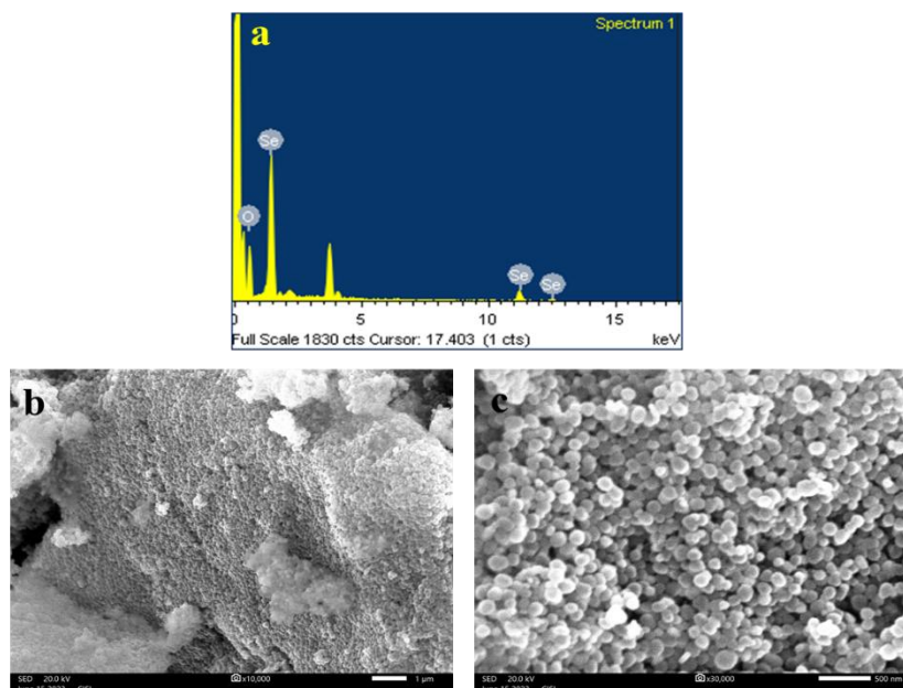
Figure 5. Characterization of SeNPs (a) Energy-dispersive spectroscopy analysis and (b) & (c) Field emission scanning electron microscopy analysis in different magnification.
