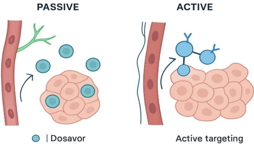
Figure 3. Tumor targeting.
