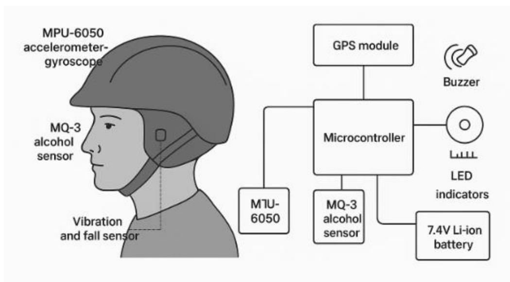
Figure 1. Overall Design Layout of the Intelligent Smart Helmet.
