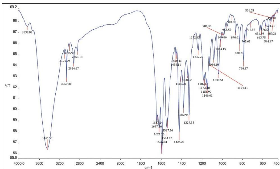
Figure 3. FTIR Spectrum of polymer Xanthun Gum.
