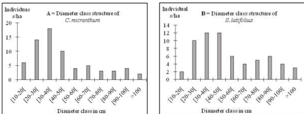
Figure 4. Diameter class structure of C. micranthum (A) and S. latifolius (B) plants.
