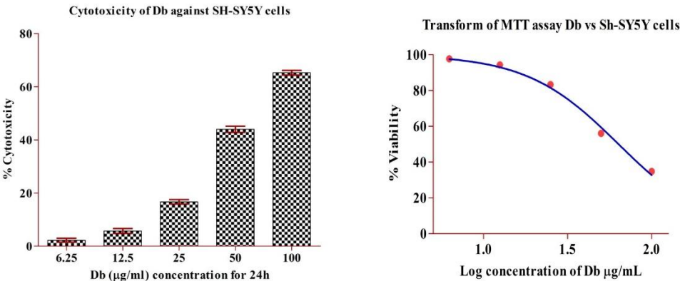
Figure 3. Dose–response curve for cytotoxicity of Dictyota bartayresiana extract on KB cells.
