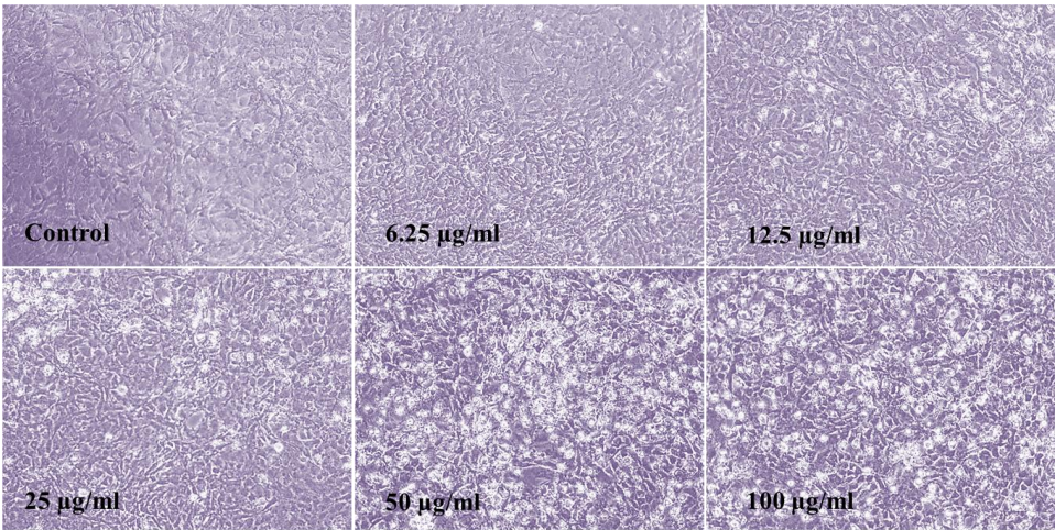
Figure 2. MTT assay showing the effect of Dictyota bartayresiana plant extract on SH-SY5Y cell viability at various concentrations (6.25, 12.5, 25, 50, and 100 \mu g/mL).
